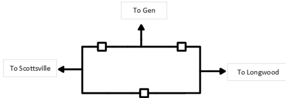
Figure 1: Point of Interconnection (POI INFORMATION) One-Line Diagram
